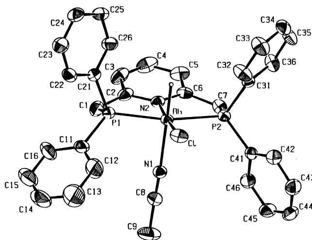
Figure 1. Platon [16] drawing of the complex cation [\text{Rh}(\text{PNP})\text{ClH}(\text{CH}_3\text{CN})]^+ of 7
